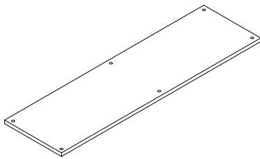
⑧ x1 955X288X12mm
