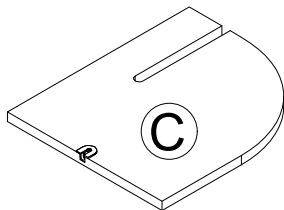
Left curved upright panel T2503847030SF
